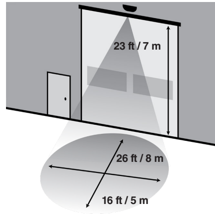
Detection area at 23 ft / 7 m height and a 45° sensor body angle
