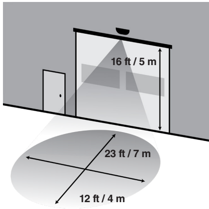
Detection area at 16 ft / 5 m height and a 45° sensor body angle
